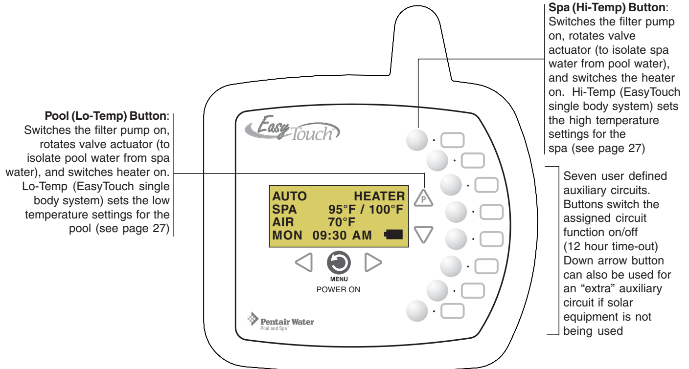
EasyTouch wireless control panel (EasyTouch 8) - (P/N 520547)
