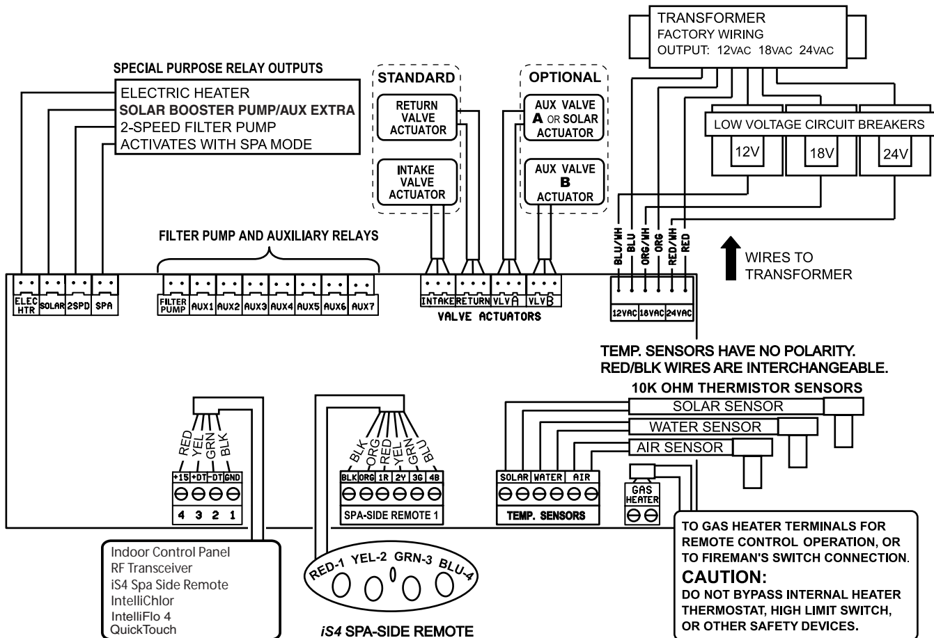
EasyTouch System Wiring Diagram (Load Center)
