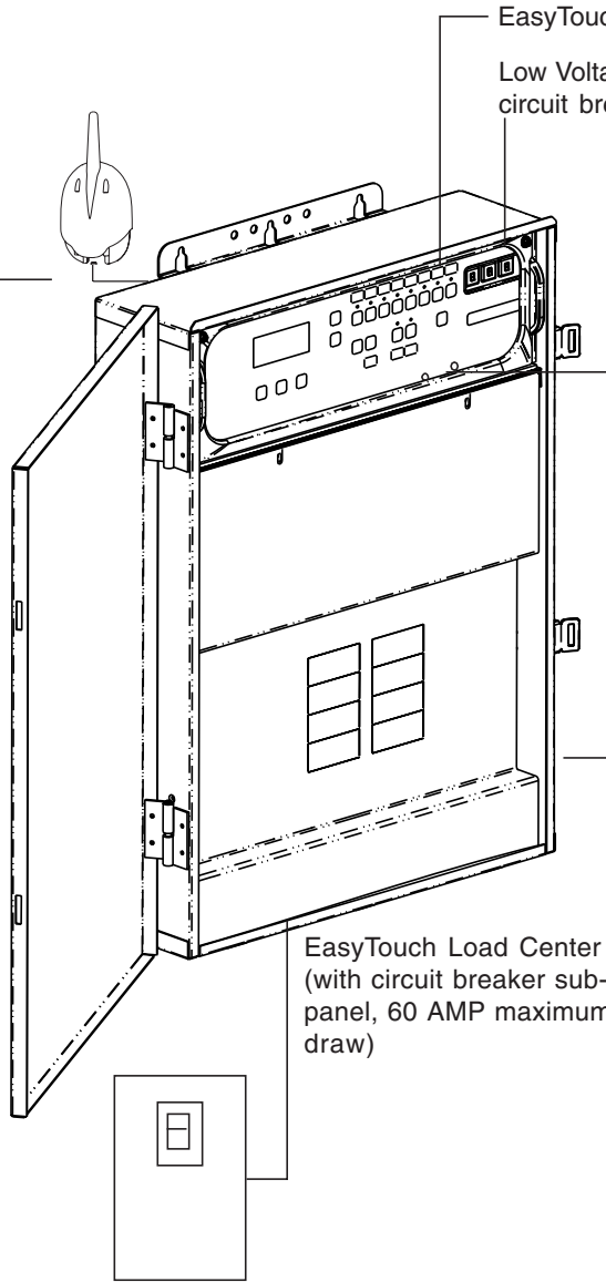
Main Power GFCI Panel 240 VAC 50 AMP (40 AMP recommended)
