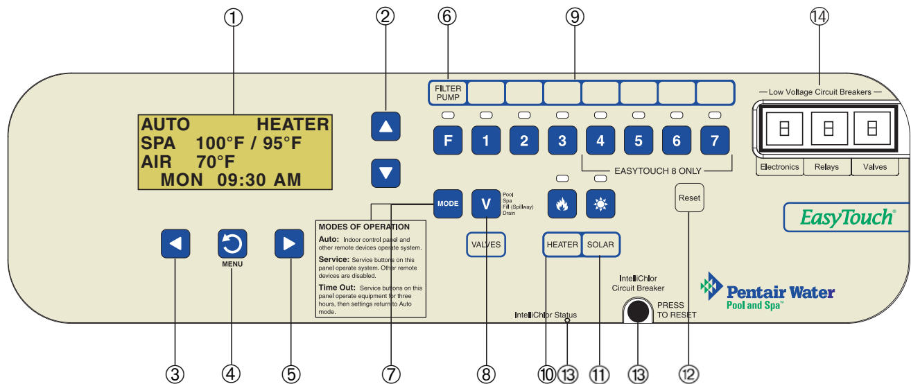
EasyTouch Outdoor Control Panel
