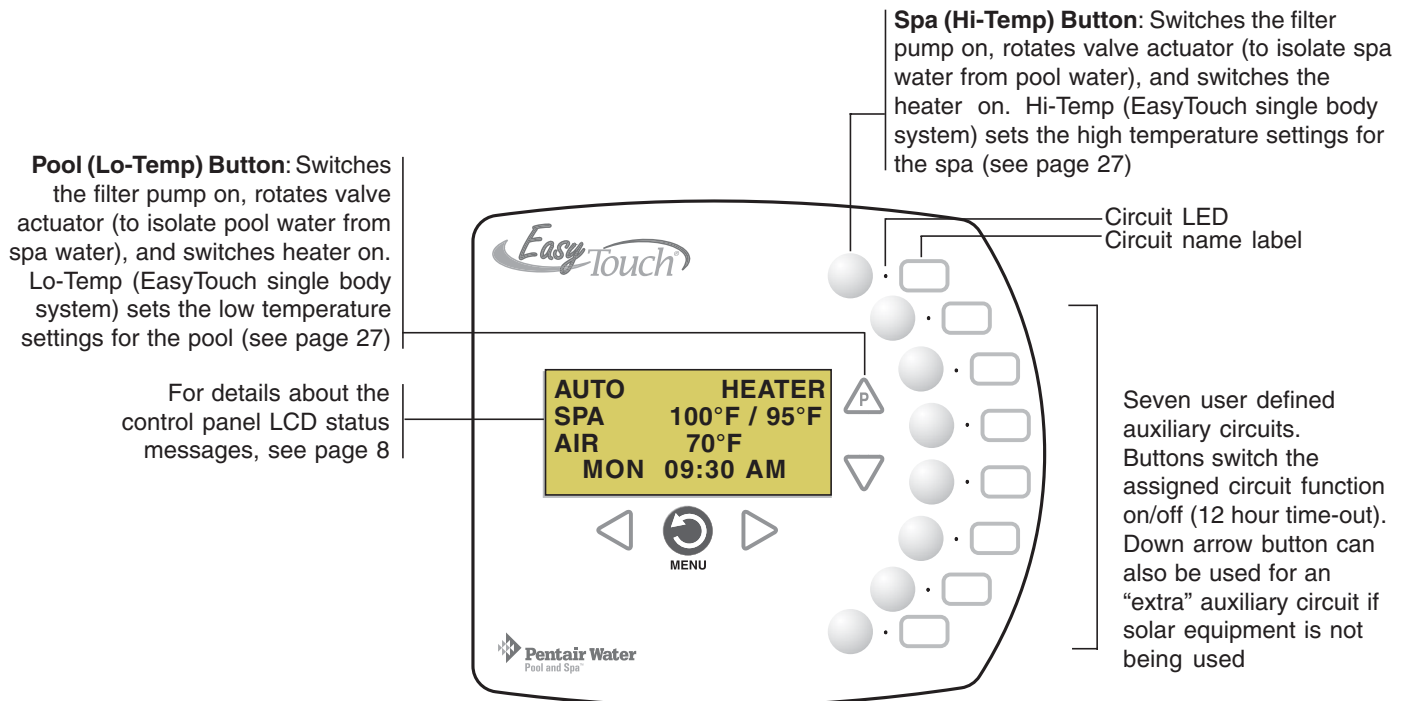
EasyTouch indoor control panel (EasyTouch 8) - (P/N 520549)
